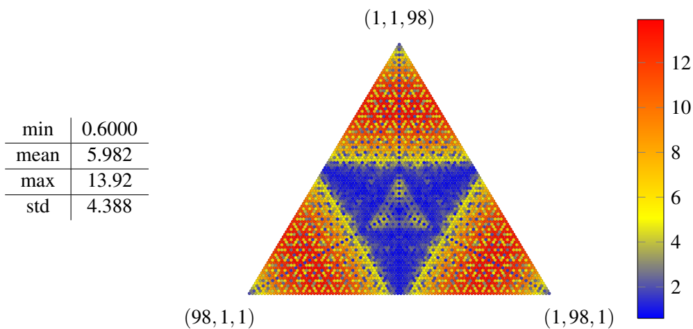
Figure 2: Discrepancy for triplets of nonnegative rational vectors (a_1/N, a_2/N, a_3/N) such that a_1 + a_2 + a_3 = N with N = 100 using Fully subtractive algorithm.
