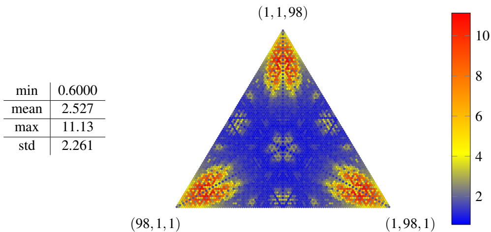
Figure 3: Discrepancy for triplets of nonnegative rational vectors (a_1/N, a_2/N, a_3/N) such that a_1 + a_2 + a_3 = N with N = 100 using Poincaré algorithm.
