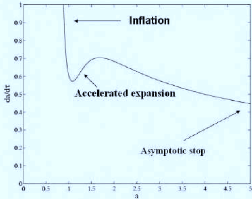
Figure 4. Expansion rate of a RW empty space-time with a defect in the origin. The behaviour includes an initial inflationary era, followed by an accelerated expansion era, and finally by a decreasing expansion rate leading asymptotically to a stop.
