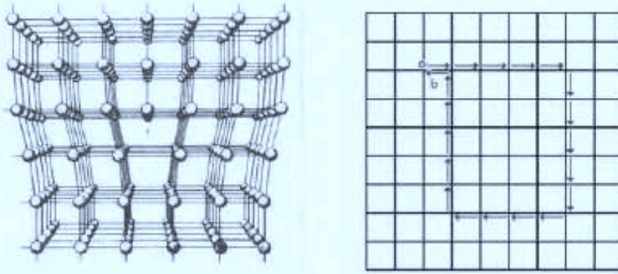
Figure 1. Schematic representation of a dislocation. The pictorial view on the left is apparently applied to a crystal, but this is absolutely not needed. On the right a closed path in the real manifold is transposed to the reference manifold evidencing the Burgers vector.
