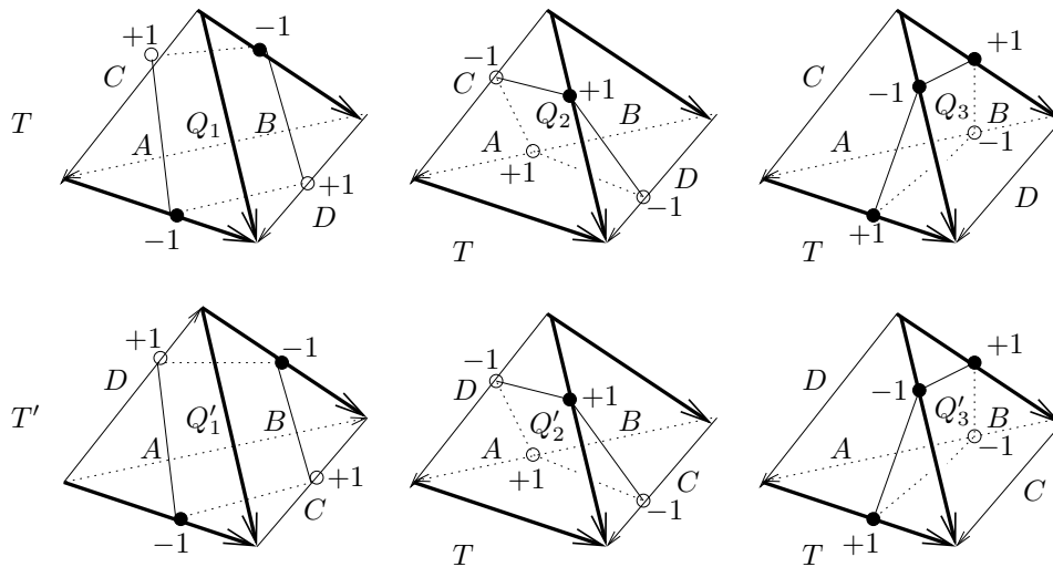
Figure 7: All quadrilateral disk types
