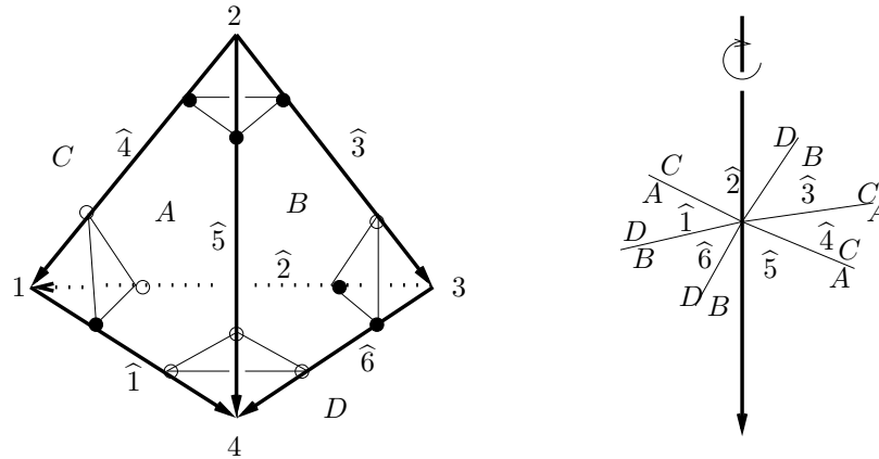
Figure 16: Gieseking manifold
