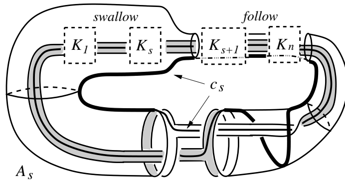
Figure 2: The Seifert Klein bottle P_s = F_n \cup A_s and center c_s \subset P_s
