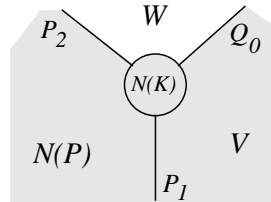
Figure 9: The manifold \widetilde{M}^3 = \widetilde{N}(P) \cup_{P_1 \cup (V \cap N(K))} V
