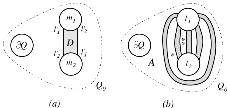
Figure 10: The possible graphs G_{Q_0}
