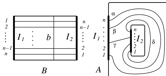
Figure 3: The arcs \omega \cap B \subset B and \omega \cap A \subset A
