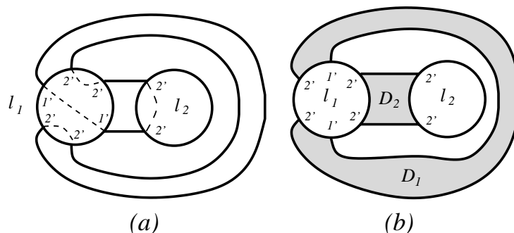
Figure 12: G_{Q_0} graphs from central intersections
