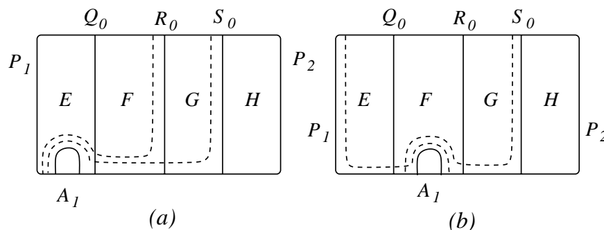
Figure 14: The possible pairs of pants T_0 (in broken lines) in H(P)
