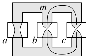
Figure 18: The pretzel knot p(a, b, c) for a = 0, b = 1, c = 1
