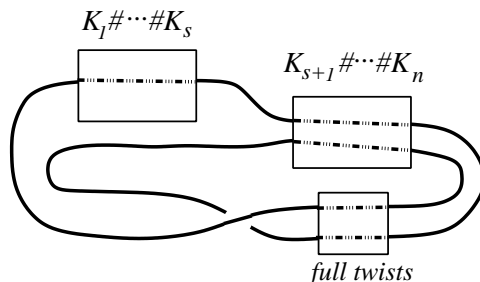
Figure 4: The knot c_s \subset S^3
