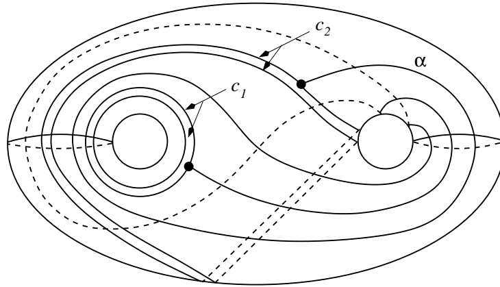
Figure 7: Coannular primitive circles c_1, c_2 in the handlebody H
