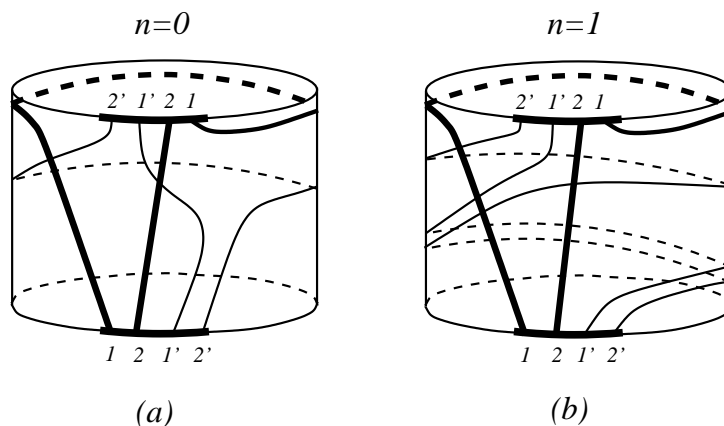
Figure 11: Minimally intersecting pairs c_1 \cup c_2, c'_1 \cup c'_2
