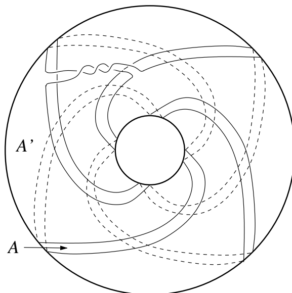
Figure 15: A modified Lyon's knot
