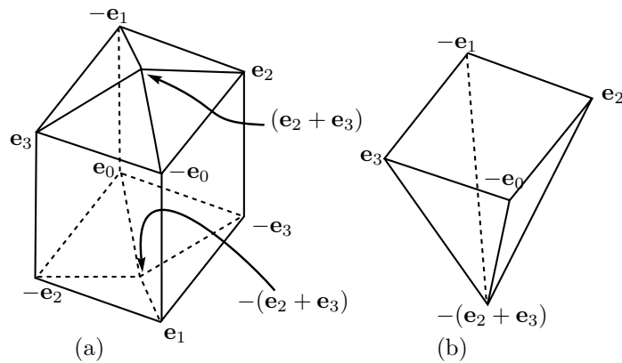
Figure 15: (a) The Thurston ball and (b) the foliation cones for Example 4
