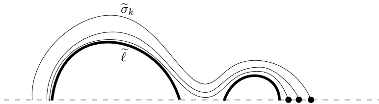
Figure 2: Nonhausdorff accumulation of \{\tilde{\sigma}_k\}_{k=1}^\infty on leaves of \tilde{\Lambda}'_+
