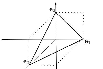
Figure 11: Foliation cones for (2, 2, 2)
