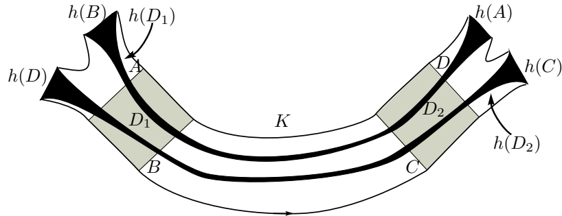
Figure 9: The core K of the leaf L of Example 1
