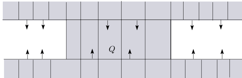
Figure 5: Opposed orientations on \partial_h Q
