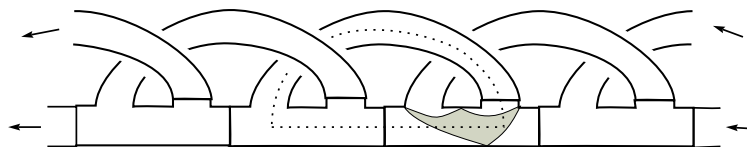
Figure 13: The leaf L of Example 3 showing the disk D_0 (shaded)
