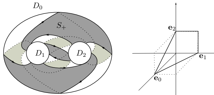
Figure 17: The sutured manifold, foliation cones, and Thurston ball for (2, 4, 2)
