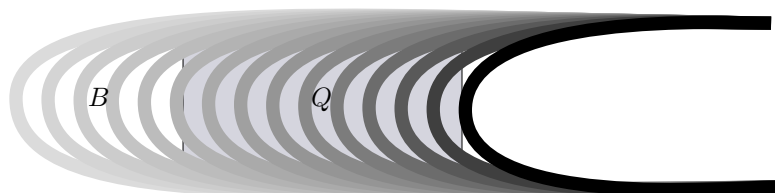
Figure 7: A complexity reducing isotopy
