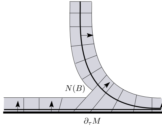
Figure 4: The normal neighborhood N(B) near \partial_\tau M
