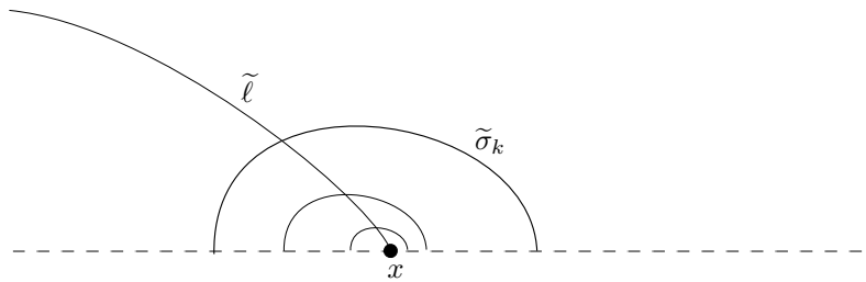
Figure 1: Each end of \tilde{\ell} limits to a point at infinity in \tilde{L}'
