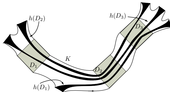
Figure 16: The core K of the leaf in Example 4
