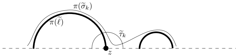
Figure 3: \pi(\tilde{\sigma}_k) crosses the geodesic \tilde{\tau}_k twice
