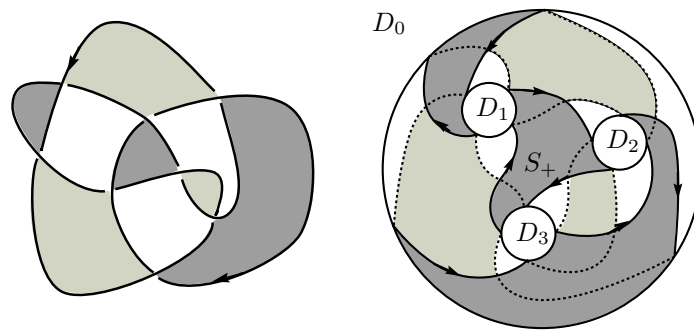
Figure 14: The 2-component link of Example 4 and the sutured manifold obtained from this link
