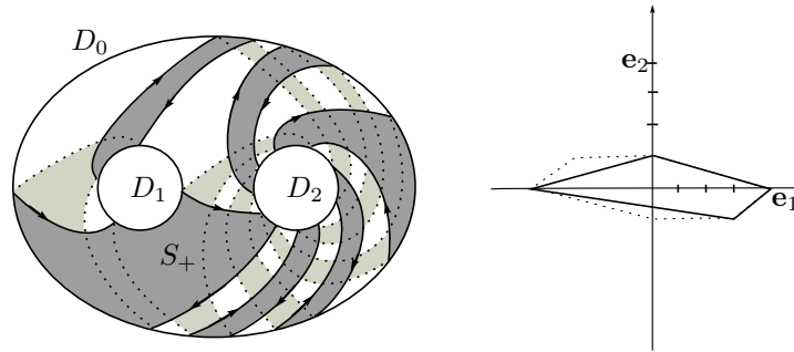
Figure 19: Example in which \{D_1, D_2\} does not work as Markov partition
