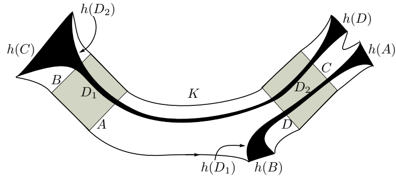
Figure 12: The core of the leaf L in Example 2
