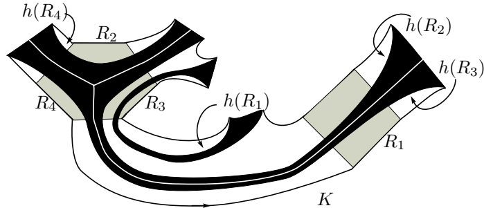
Figure 18: The core K of the leaf in Example 5
