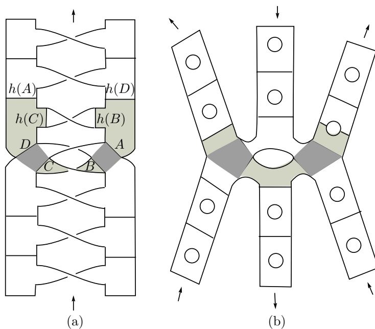
Figure 10: (a) The leaf L of Example 1 (b) The leaf L of Example 2
