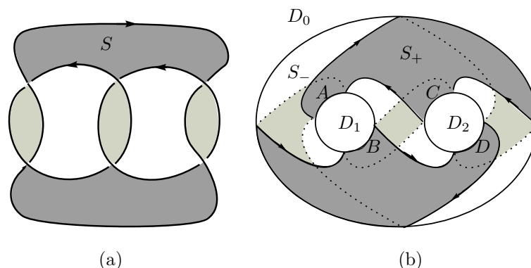
Figure 8: (a) A Seifert surface for (2, 2, 2) (b) The sutured manifold M obtained from (2, 2, 2)
