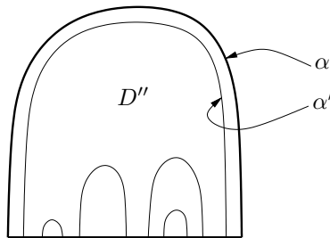
Figure 10: The disk D , showing D \cap H and D''
