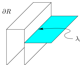
Figure 12: A cross-sectional view of \partial R ( \Delta_F shaded)
