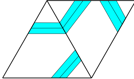
Figure 11: A bit of \Theta_F with the nearby \Theta_Y shaded
