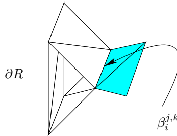
Figure 14: Triangulation of \partial R near \beta_i^{j,k} ( \Delta_F shaded)
