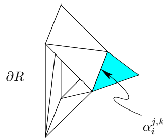
Figure 13: Triangulation of \partial R near \alpha_i^{j,k} ( \Delta_F shaded)
