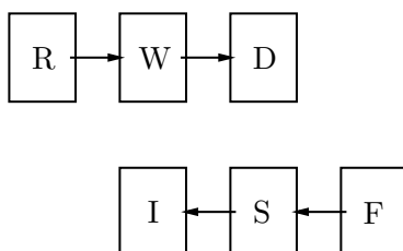
Figure 1: Reducibility implies weakly reducibility which in turn implies the DCP. Also fullness implies strong irreducibility which in turn implies irreducibility. It is an amusing exercise to find a Heegaard splitting for every column.
