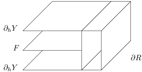
Figure 9: Side-view of F \subset Y
