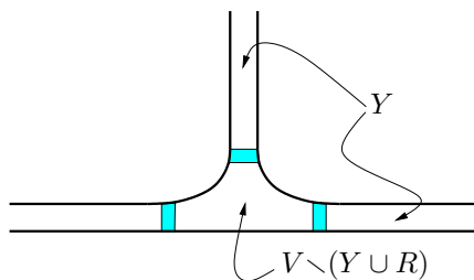
Figure 8: A cross-section of V . The union of tori, R , is shaded.
