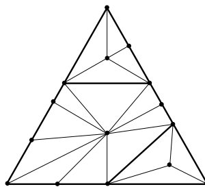
Figure 15: The subdivision of a face \sigma
