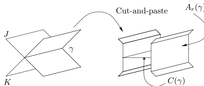
Figure 5: The exchange band for \gamma
