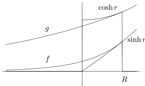
Figure 1: Constructing a negatively curved metric
