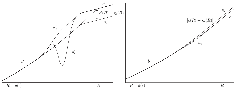
Figure 3: Smoothing a' and a
