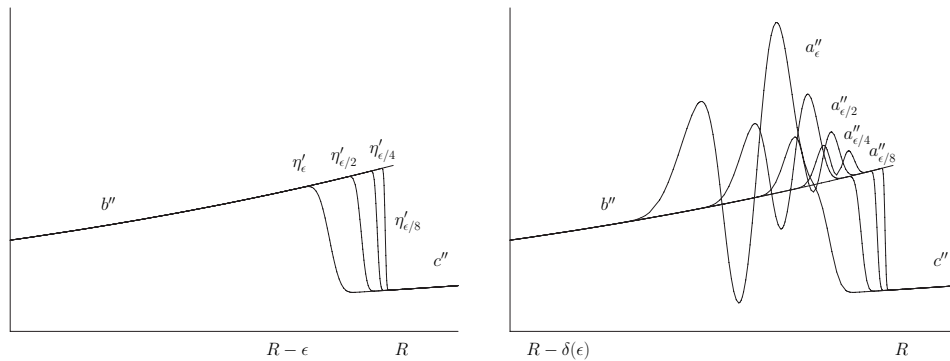
Figure 2: Interpolating between b'' and c''
