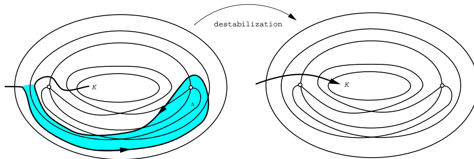
Figure 9: K enters into the foliated region and intersects a singular leaf twice. This allows for a destabilization of K . The shaded region corresponds to the of Lemma 2.5.
