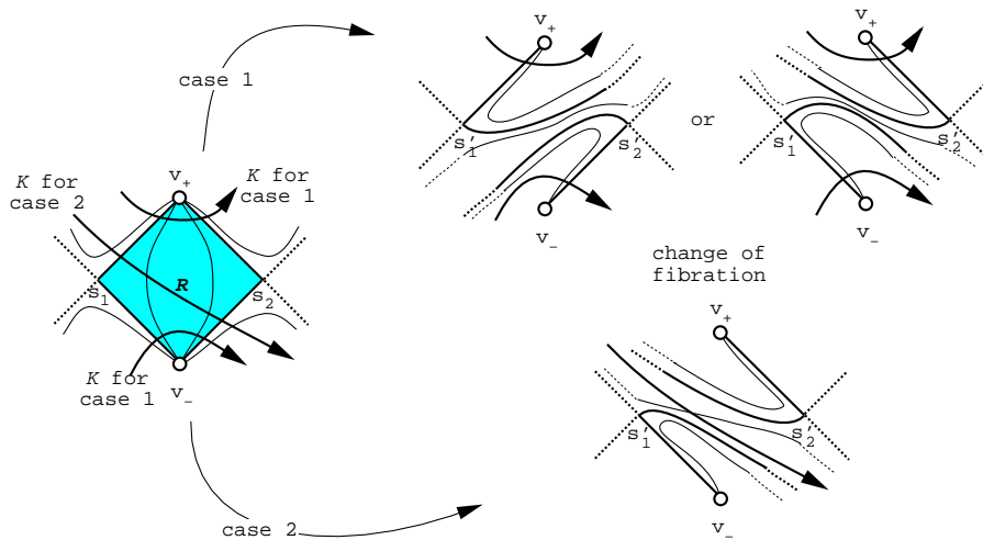
Figure 5: Parity of s_1 equals parity of s_2 . In case 1 there are two possible ways to change the fibration of H and, thus, the foliation of T . In case 2 there is only one way to alter the fibration.
