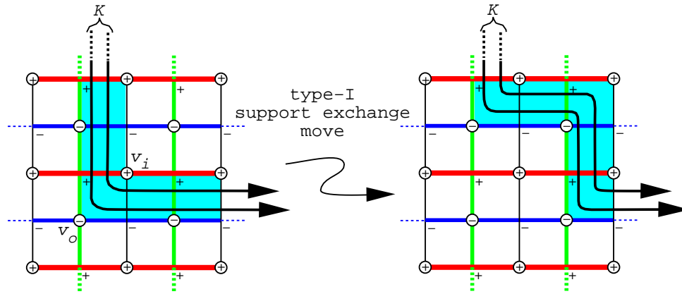
Figure 11: The alteration in S_K from left to right corresponds to an exchange move with type-I support. The vertex labeled v_o is an outside vertex and the vertex labeled v_i is an inside vertex. The shaded region is a portion of S_K .
