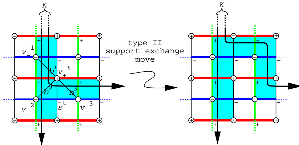
Figure 12: The alteration in S_K from left to right corresponds to an exchange move with type-II support. The vertex labeled v^t is a tee vertex and the singularity labeled s^t is a tee singularity. The shaded region indicates a portion of S_K .
