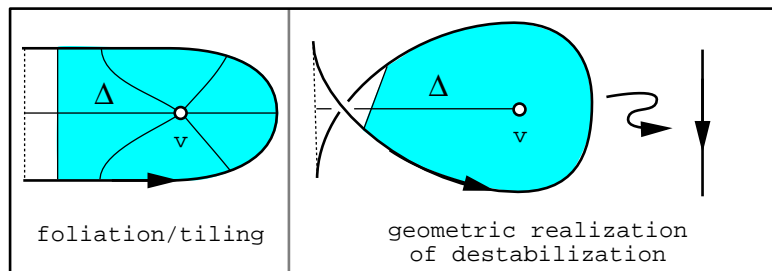
Figure 3: The vertex v has type (a).
