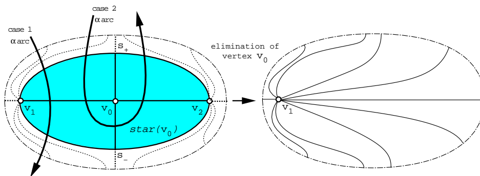
Figure 6: The vertex v_0 is a type (b,b) vertex. In the situation where the case 2 arcs are absent, after an exchange move, the \mathbf{b} {arcs between v_0 and v_2 are inessential.
