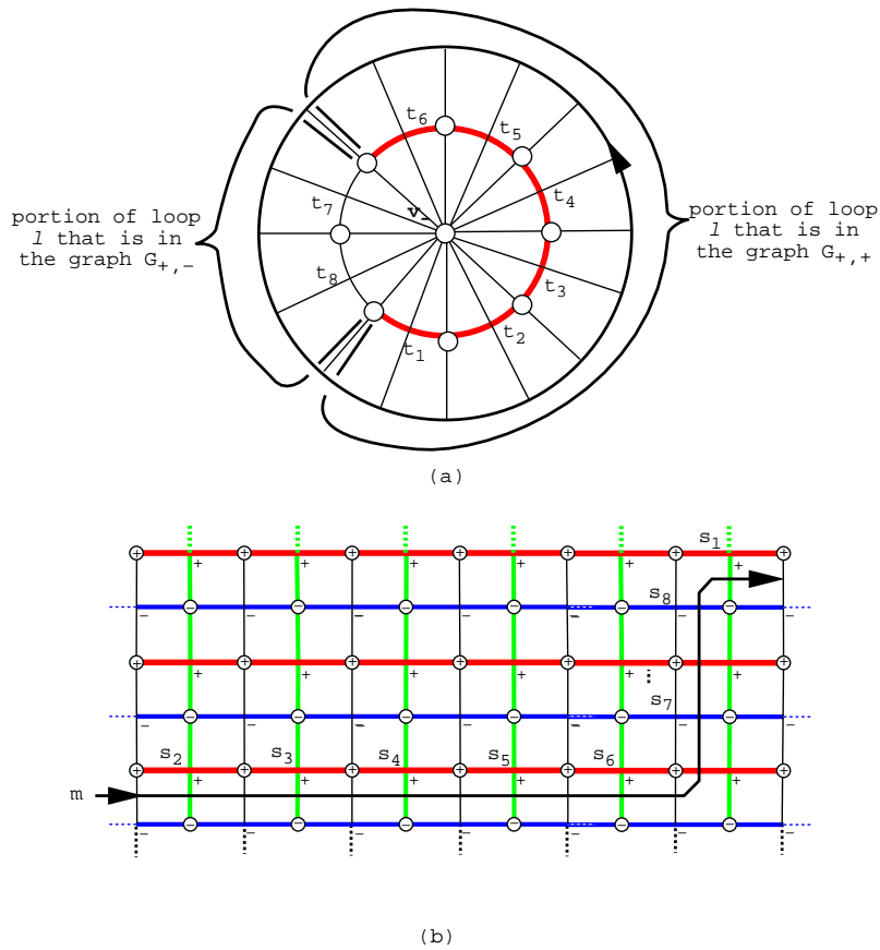
Figure 14: In (a) we have the foliation of m illustrated in the special case where l contains two negative and six positive singularities, and there is a single negative vertex. In (b) we have the corresponding path m in a standard tiling of T . The arrowheads are identified to form a scc. The labels t_1; \dots; t_8 of the singularities in (a) show the sequential correspondence to the singularities in (b) with the labels s_1; \dots; s_8 .
