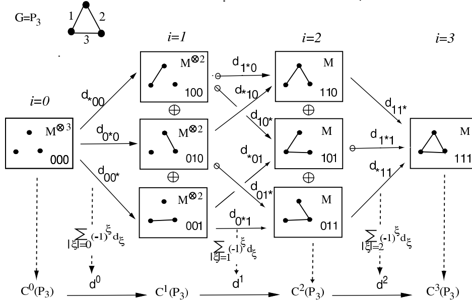
Figure 4: The differentials
