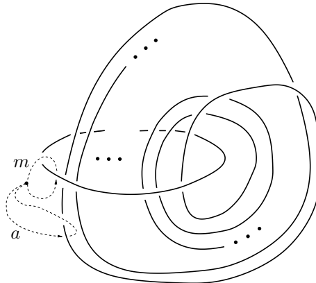
Figure 1: The link L_n
