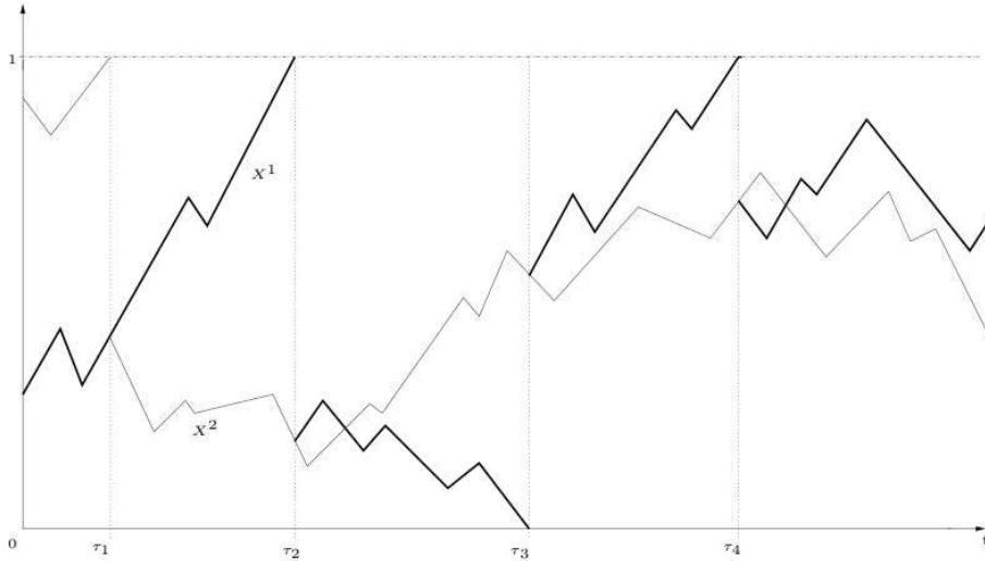
FIG 12. Fleming-Viot type system with two particles absorbed in 0 and 1.
