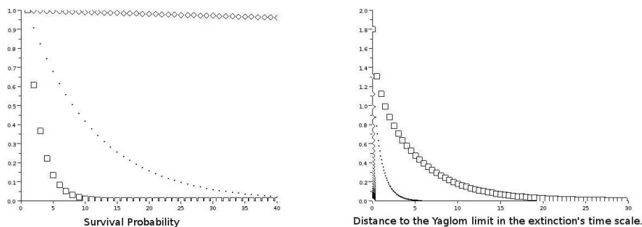
FIG 1. Example 1. A numerical computation leads to \lambda = 9.8 \times 10^{-4} . Three different situations are observed, which lead to three very different patterns for the speed of convergence to the Yaglom limit in the extinction's time scale: ( \diamond ) \lambda \gg d = 0.1 \times 10^{-4} ; ( \square ) \lambda \ll d = 50 \times 10^{-4} ; ( \cdot ) \lambda = d = 9.8 \times 10^{-4} .
