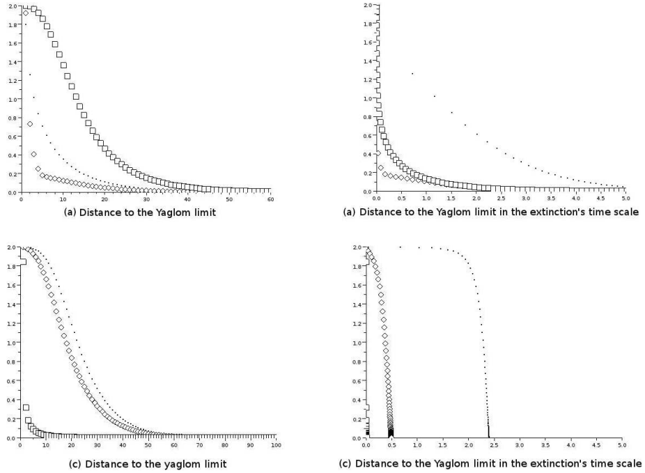
FIG 3. Example 2. Pictures (a) and (c) correspond to different values of \lambda (the following values of \theta(\alpha) - \chi have been obtained by numerical computation): (a) \lambda = 0.9 , \theta(\alpha) = 0.100 , \theta(\alpha) - \chi = 0.102 ; (c) \lambda = 1.1 , \theta(\alpha) = 5.84 \times 10^{-5} , \theta(\alpha) - \chi = 0.103 ; each curve corresponds to a given initial size of the population: (\cdot) Z_0 = 1 ; (\diamond) Z_0 = 10 ; (\square) Z_0 = 100 .
