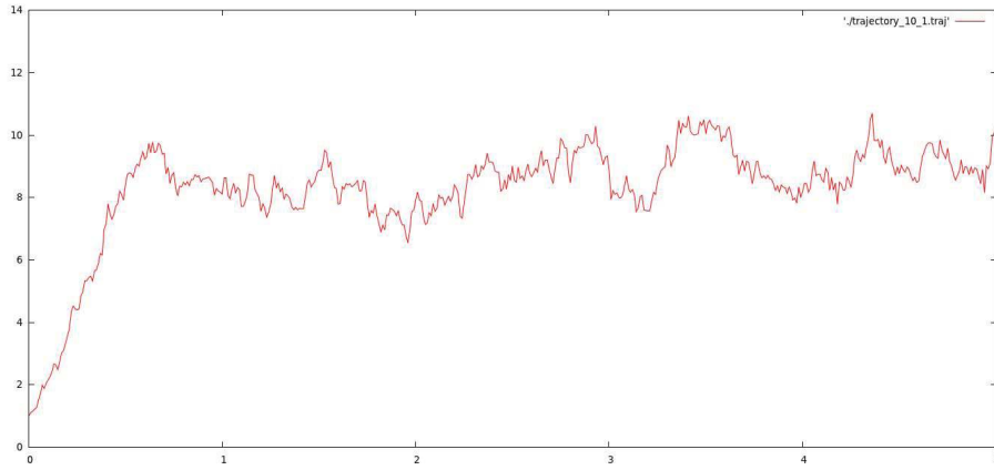
FIG 7. Example 4. A random path for logistic Feller diffusion process with initial size Z_0 = 1 and parameters r = 9 and c = 1
