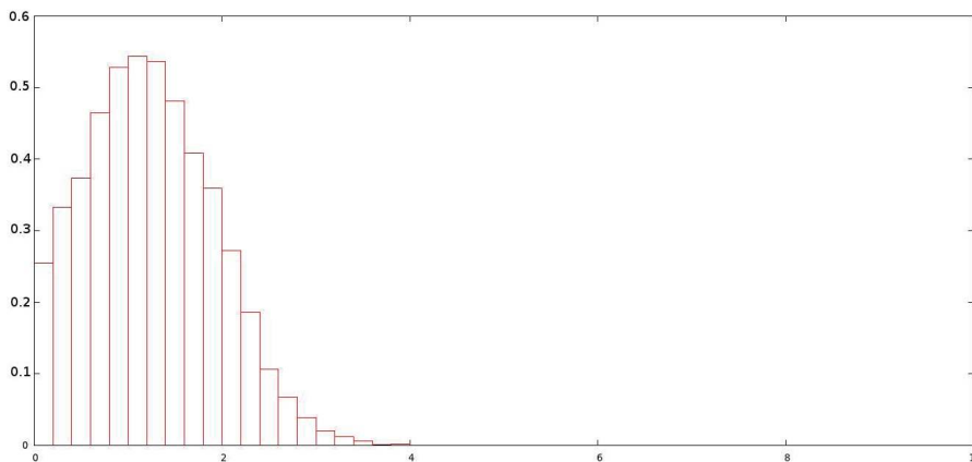
FIG 11. First marginal of the Yaglom limit of a 3-type stochastic Lotka-Volterra system. The two other marginals are equal to the null measure.
