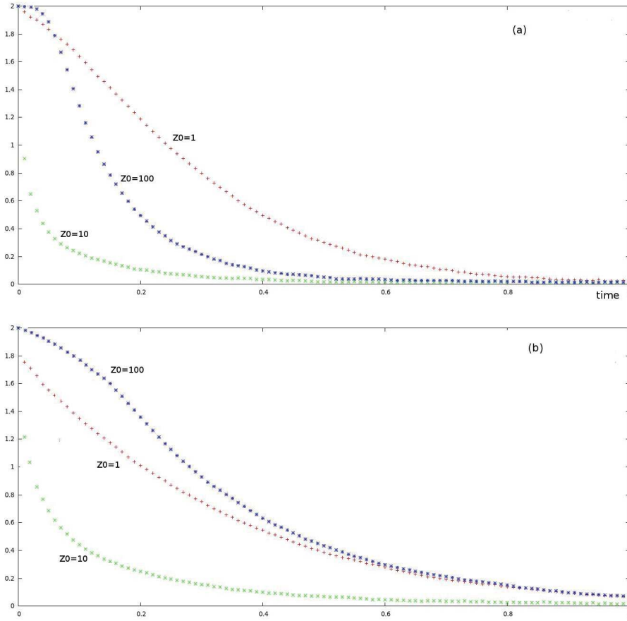
FIG 6. Example 3. Evolution of the distance between the conditioned distribution and the Yaglom limits of two logistic birth and death processes with the same charge capacity \frac{\lambda-\mu}{c} = 9 : (a) \lambda = 10 , \mu = 1 and c = 1 ; (b) \lambda = 10 , \mu = 7 and c = 1/3 .
