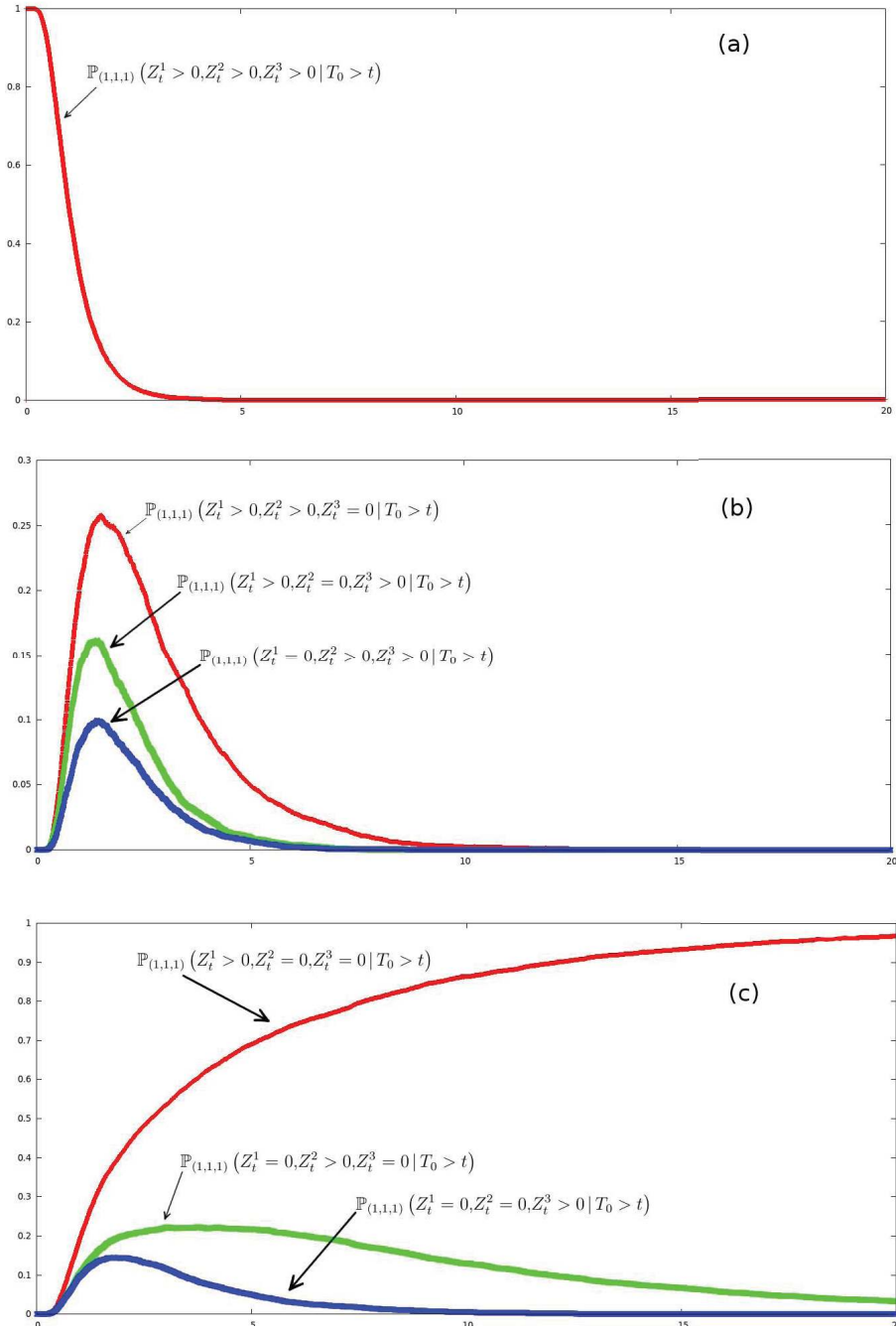
FIG 10. Dynamics of the probabilities of co-existence and existence of the different types for a 3-type stochastic Lotka-Volterra system. The horizontal axis is the time axis
