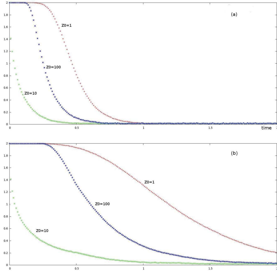
FIG 9. Example 4. Evolution of the distance between the conditioned distribution and the Yaglom limits of two logistic Feller diffusion processes with the same charge capacity \frac{r}{c} = 9 : (a) r = 9 and c = 1 ; (b) r = 3 and c = 1/3 .
