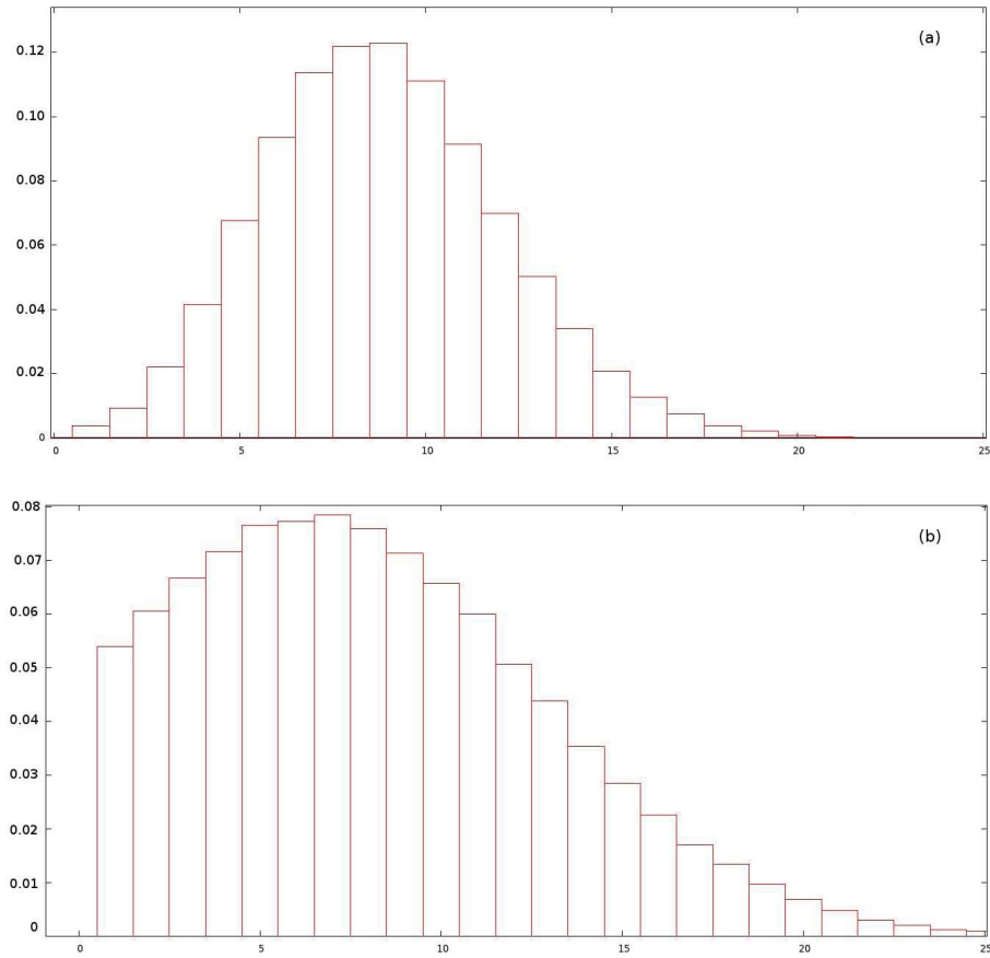
FIG 5. Example 3. The Yaglom limits of two logistic birth and death processes with the same charge capacity \frac{\lambda-\mu}{c} = 9 : (a) \lambda = 10 , \mu = 1 and c = 1 ; (b) \lambda = 10 , \mu = 7 and c = 1/3 .
