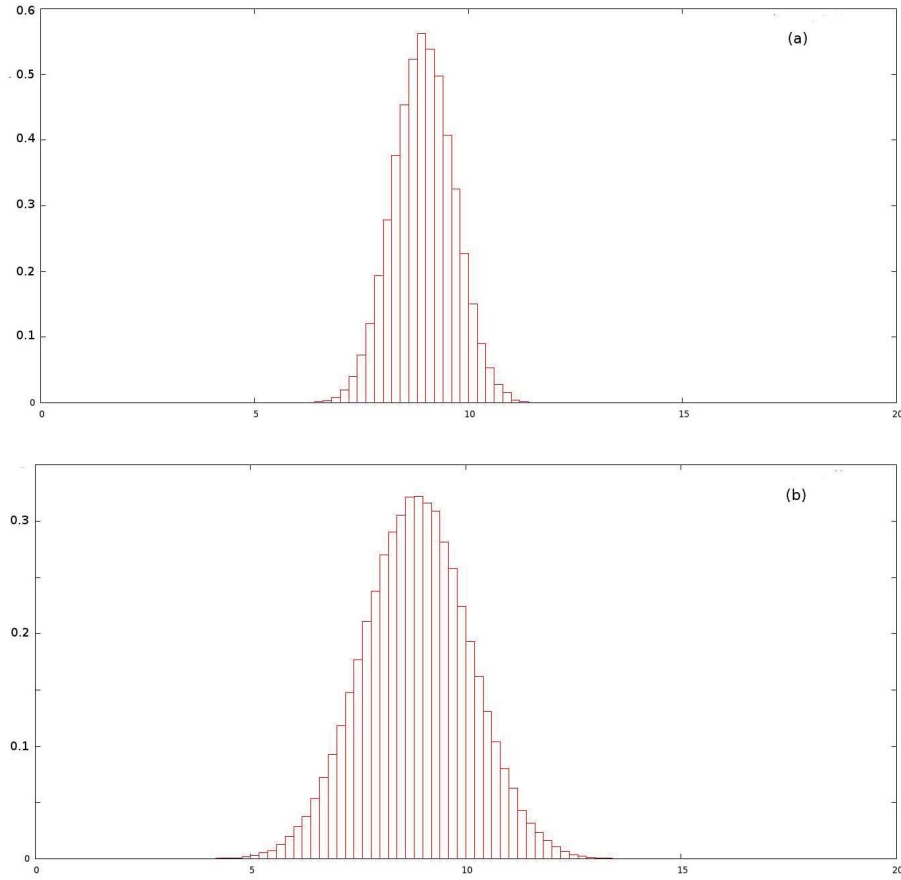
FIG 8. Example 4. The Yaglom limits of two logistic Feller diffusion processes with the same charge capacity: (a) r = 9 and c = 1 ; (b) r = 3 and c = 1/3 .
