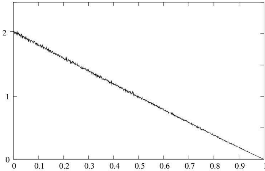
FIG 13. The Yaglom limit of the Wright-Fisher diffusion conditioned to be absorbed at 0 obtained by numerical simulation.
