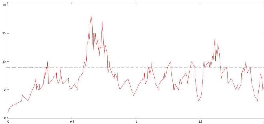
FIG 4. Example 3. A random path of a logistic birth and death process with initial size Z_0 = 1 and with parameters \lambda = 10 , \mu = 1 and c = 1
