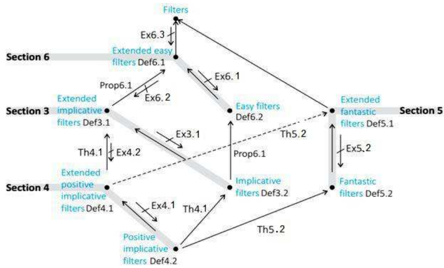
FIGURE 1. The relationship between filters in triangle algebra
