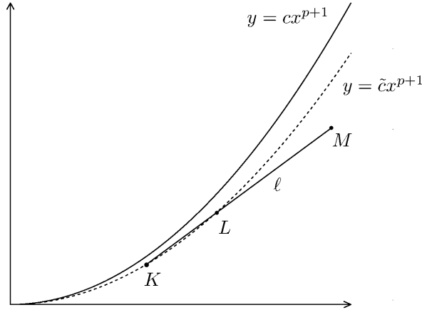
FIGURE 1. The crucial points and their geometric interpretation: K = (1 - \delta, \tilde{c}(1 - \delta)^{p+1}) and L = (1, \tilde{c}) lie on the curve y = \tilde{c}x^{p+1} , the point M = \left( 1 + \eta, \tilde{c} \left( 1 + \eta \cdot \frac{1 - (1 - \delta)^{p+1}}{\delta} \right) \right) lies on the line \ell .
