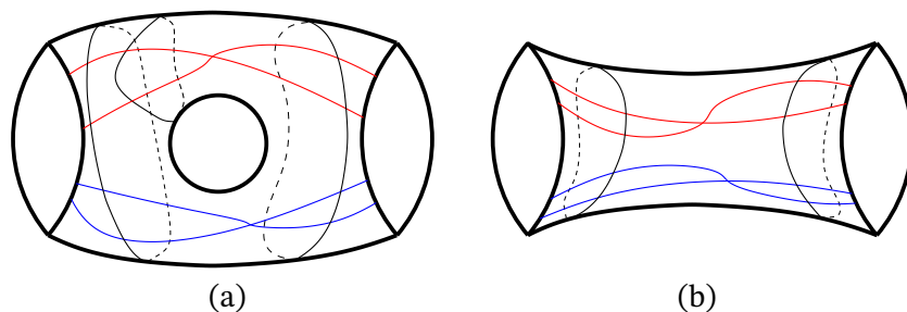
FIGURE 3. In both (a) and (b), an alternating link diagram is projected on the surface F , shown on a part of F which disconnects the surface. In both cases, the red crossing and the blue crossing are homologically twist-equivalent. One of the Tait graphs in (a) has homologous loops, and in (b) has a null-homologous 2-cycle. Neither pair of crossings forms a twist region on F .
