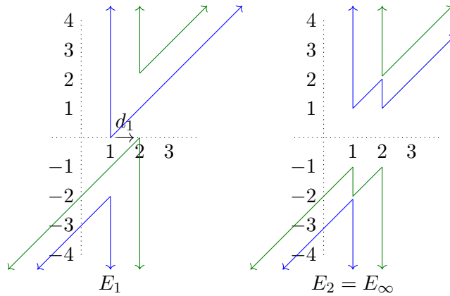
FIGURE 13. Jack-O-lantern modules in a spectral sequence.
