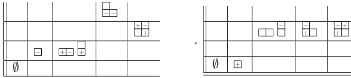
FIGURE 20. Ingredients tables I(- + - +) and I(+ - - +) for \text{Gr}_2(\mathbb{R}^{4,2}) .
