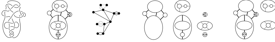
FIGURE 1. Left to right: a link diagram D with a homogeneously adequate state x , its graph G_x , blocks, and zones.
