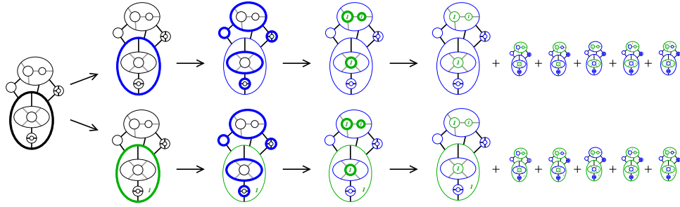
FIGURE 7. Constructing X^\pm \in \mathcal{C}_{\mathbb{F}_2}(x) , as in the direct proof of the main theorem.
