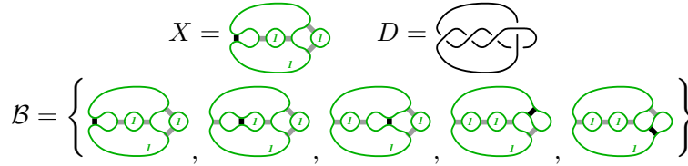
FIGURE 10. Over \mathbb{F}_2 , this enhancement X of an inessential state x of D represents a nonzero homology class, since dX = 0 and \varepsilon \circ \pi_{\mathcal{B}} \circ d \equiv 0 , where \mathcal{B} is an \mathbb{F}_2 -basis for \mathcal{C}_{\mathbb{F}_2}^{i_x, j_X}(D) .
