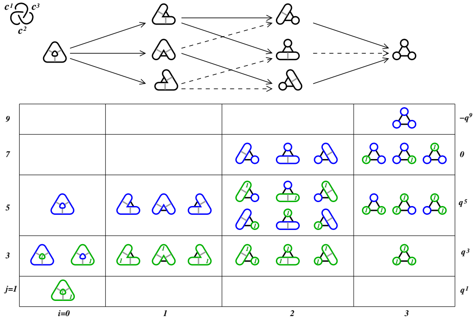
FIGURE 2. The Jones polynomial V_L(q) = q + q^3 + q^5 - q^9 of the RH trefoil via Khovanov chains.
