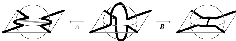
FIGURE 4. Use crossing balls C = \bigsqcup C^t to embed a link and its states' circles in (S^2 \setminus C) \cup \partial C .
