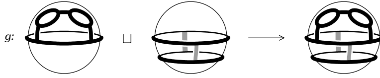
FIGURE 5. A gluing map g : (S^2, x) \sqcup (S^2, y) \rightarrow (S^2, z) for a plumbing of states x * y = z .
