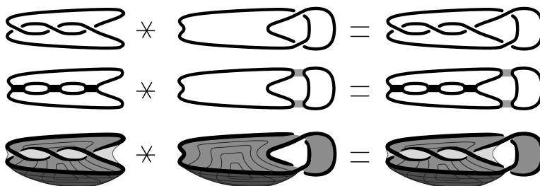
FIGURE 6. Plumblings of link diagrams, states, and surfaces.
