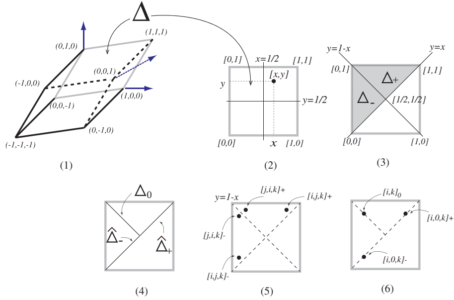
FIGURE 5. (1) Thurston norm ball U_N and the fibered face \Delta . (2) [x, y] \in \Delta . (3) \Delta_{\pm} . (4) \Delta_0, \widehat{\Delta}_{\pm} . (5) Projective classes [i, j, k]_{\pm} and [j, i, k]_{\pm} . (6) Projective classes [i, 0, k]_{\pm} and [i, k]_0 = [0, i, k]_{\pm} .
