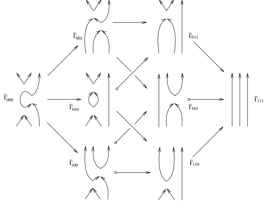
FIGURE 3. The cube of resolutions of D_3 .
