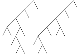
FIGURE 5. Tree pair diagram for \psi^2(w) = x_0^4 x_1 x_4 x_3^{-1} x_2^{-2} x_0^{-3} , where the word w = x_0^2 x_1 x_3^{-1} x_2^{-1} x_0^{-1} is depicted in Figure 3.
