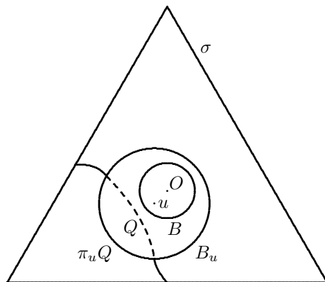
Figure 1: Projecting Q to the boundary of B_u .
