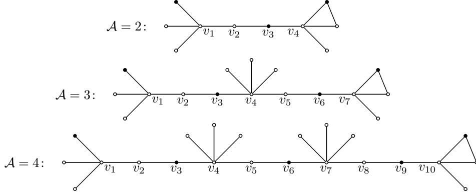
Figure 7. The graph G for \mathcal{A} = 2, 3, 4 .
