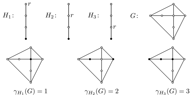
Figure 1. A minimum H_i -dominating set ( i = 1, 2, 3 ) for a graph G .
