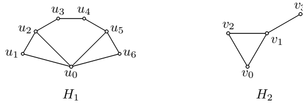
Figure 3. The graphs H_1 and H_2 .
