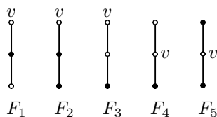
Figure 2. The five 2-stratified graphs P_3 .
