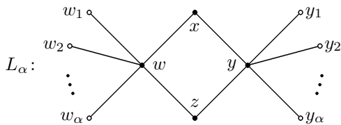
Figure 6. The graph L_\alpha .
