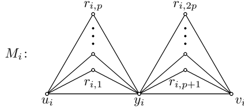
Figure 4. The graph M_i .
