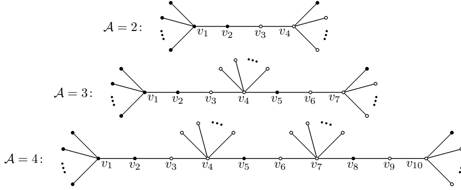
Figure 5. The graph G for \mathcal{A} = 2, 3, 4 .
