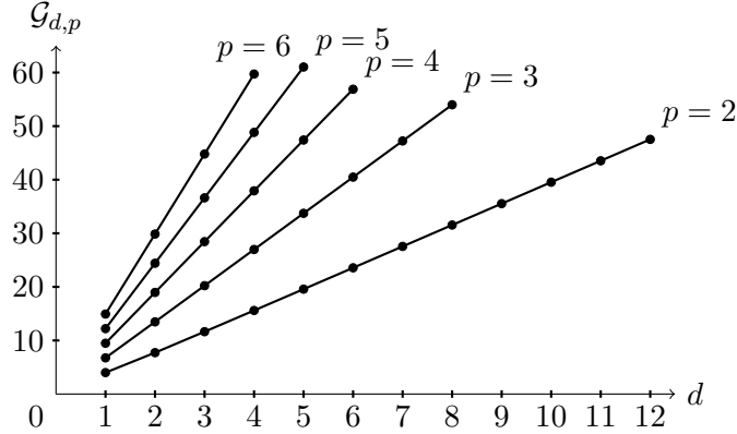
Figure 3: The growth rate \mathcal{G}_{d,p} for various d and p
