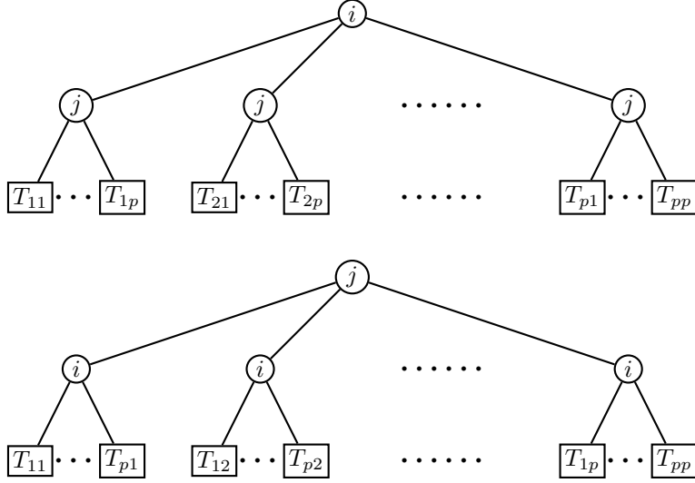
Figure 6: Two interchange equivalent trees
