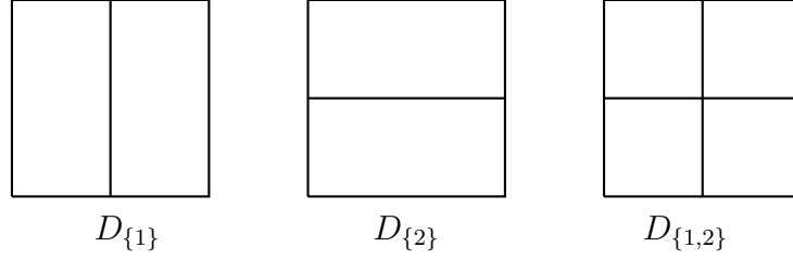
Figure 4: Illustrating the definition of D_S in the case of d = p = 2
