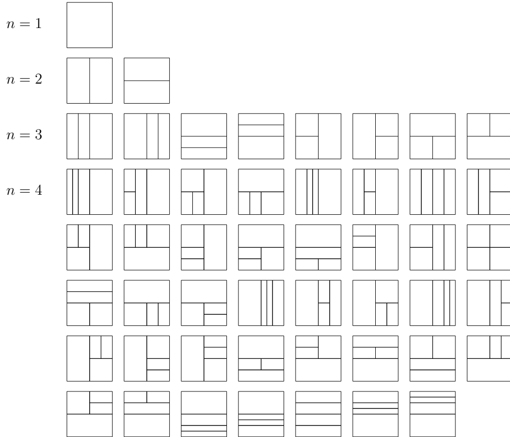
Figure 1: Decompositions of the unit square ( d = 2 ) using bisections ( p = 2 ) into n \leq 4 subrectangles
