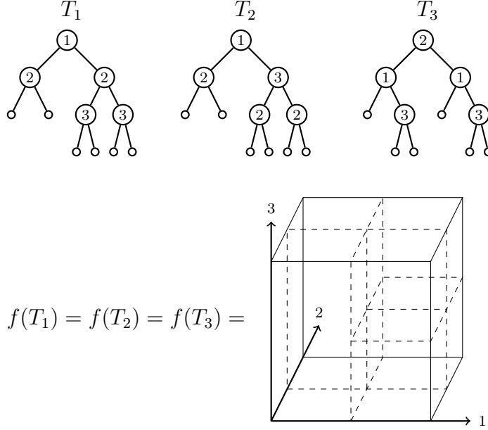
Figure 5: Example of the map f from trees to decompositions (Definition 13)
