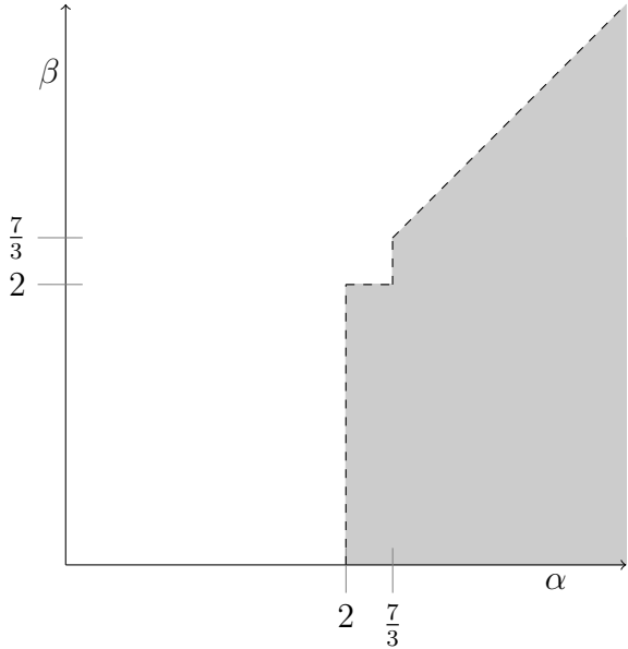
Figure 1: Conjecture for k = 2 ( \mathfrak{S}_2 in grey.)
