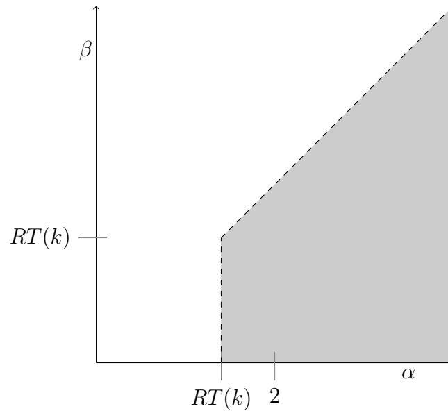
Figure 2: Conjecture for k \geq 3 ( \mathfrak{S}_k in grey.)
