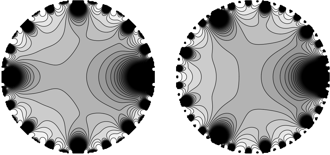
Figure 4: Contour plots of |\underline{\Lambda}_{2,2}(y)| on the left and |\Lambda_{3,3}(y)| on the right, both on the open unit disk |y| < 1 , with dark shading indicating large values.
