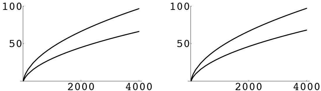
Figure 5: Least square fits to points (n, \log(\lambda_{2,2^j,n}/c_{2,2^j}(n))) on the left and (n, \log(\lambda_{3,3^j,n}/c_{3,3^j}(n))) on the right, for j \in \{1, 2\} and 20 \leq n \leq 4000 .
