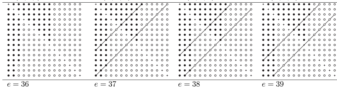
Figure 9: Adjacency matrices for quasi-complete and quasi-star graphs with v = 15 and 36 \leq e \leq 39
