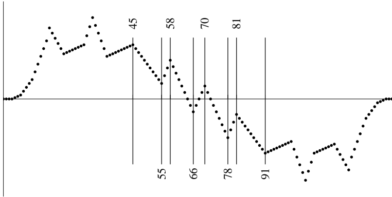
Figure 7: S(17, e) - C(17, e) > 0 for 4 \leq e \leq 63 .
