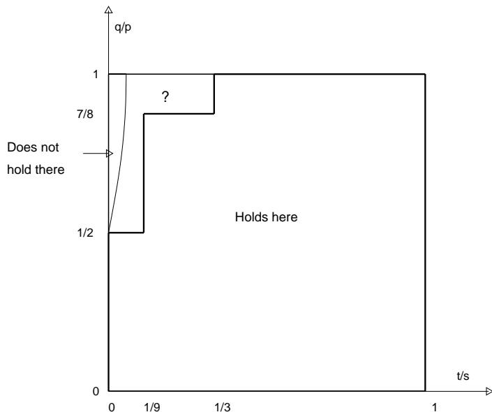
Figure 2: When does G_{s,t} \succeq E_{p,q} hold?
