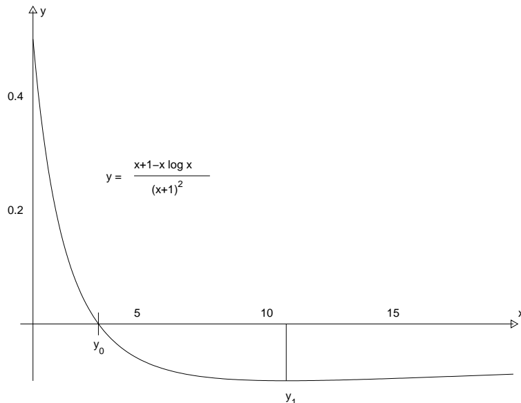
Figure 1: The function h .
