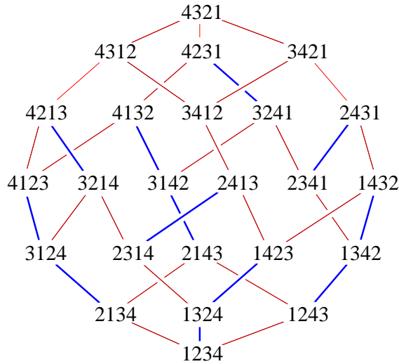
Figure 1: The fibers of P_1 : S_4 \rightarrow S_3 \times S_2
