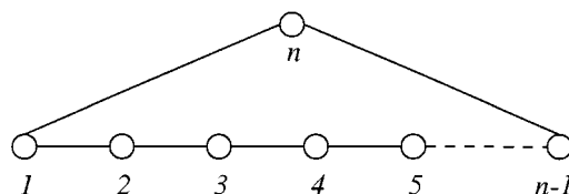
Figure 1. Dynkin diagram of type \tilde{A}_{n-1} .
