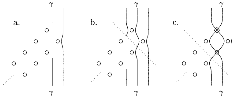
Figure 16. It is clear that \gamma must remain in its column in order for \pi(w^\sigma) = e . This is shown in (a). Diagrams (b) and (c) show the only two possibilities for the path of \gamma .
