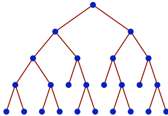
Figure 5: The tree for l = 13
