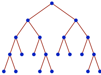
Figure 4: The tree for l = 11
