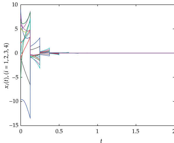
Figure 2: Evolution of the state variable x_i(t) , i = 1, 2, 3, 4 .
