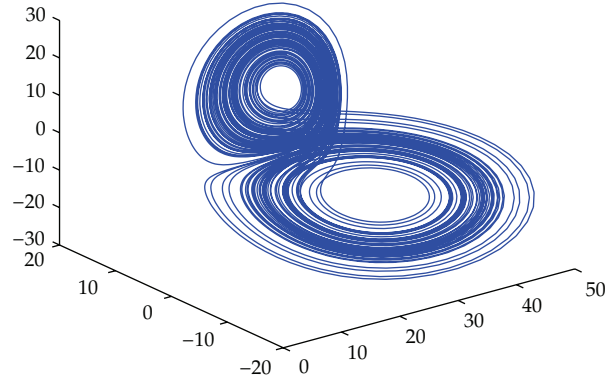
Figure 1: The double-scroll attractor of the Lorenz system.
