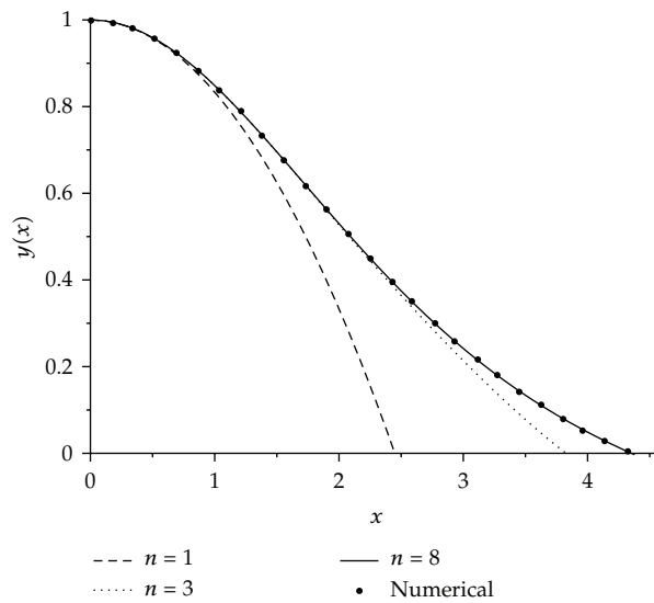
Figure 2: Solutions of the Lane-Emden equation at different orders of the MSLM approximate solution.
