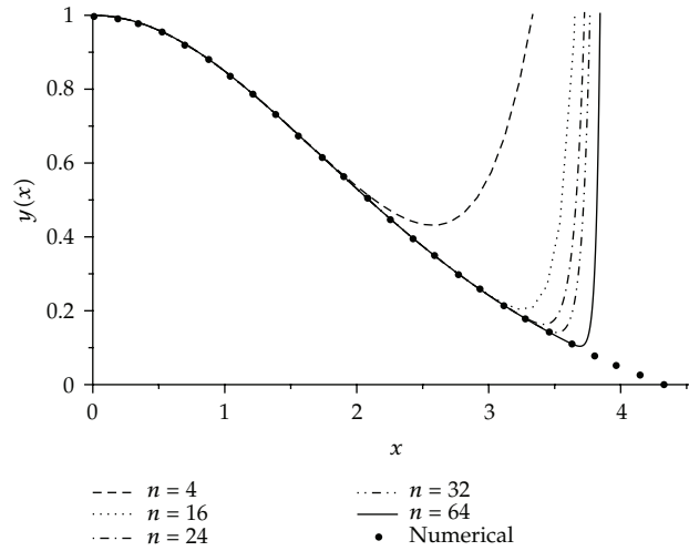
Figure 1: Solutions of the Lane-Emden equation at different orders of the ADM approximate solution.
