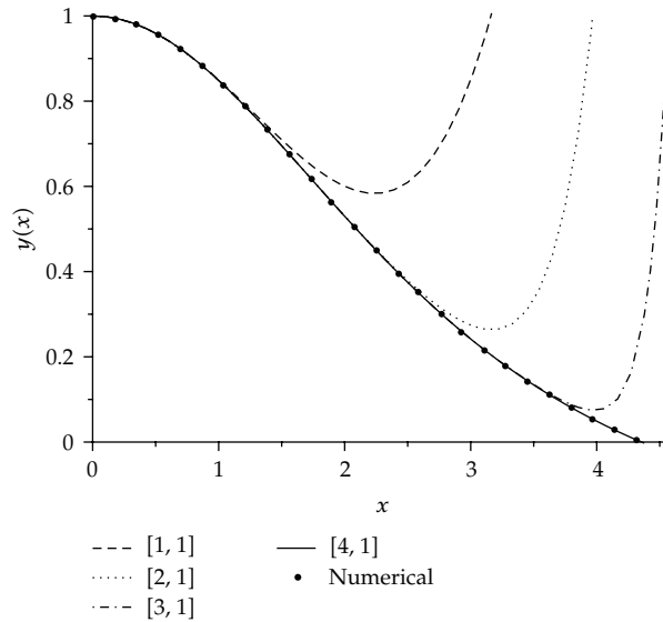
Figure 3: Solutions of the Lane-Emden equation at different orders of the SLM-ADM approximate solution.
