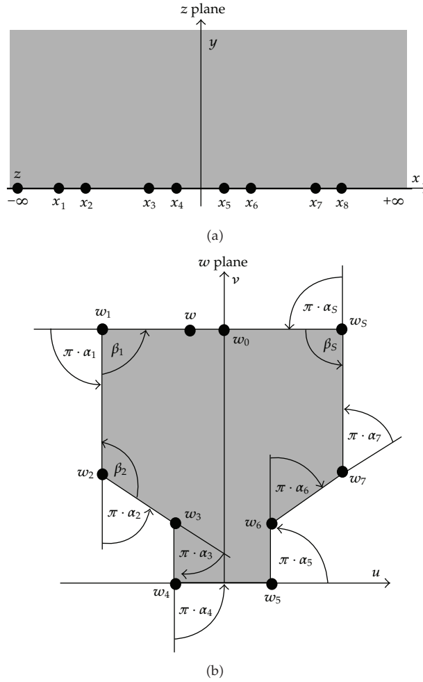
Figure 1: Mapping of a polygon through the direct Schwarz-Christoffel transformation.
