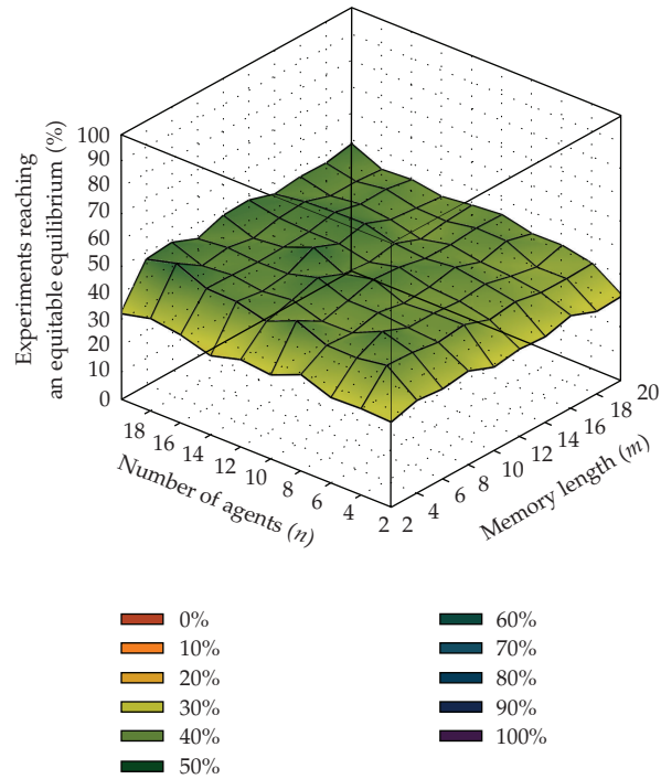
Figure 5: Percentage of experiments that reached an equitable equilibrium as the first centre of attraction. Uncertainty parameter \epsilon = 0.2 . New decision rule.
