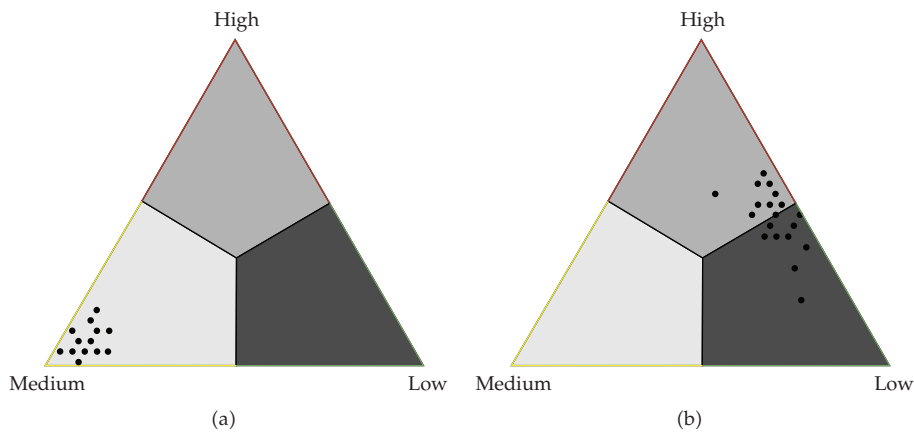
Figure 6: Modification of AEY’s model with a new decision rule. Number of agents n = 100 , uncertainty parameter \epsilon = 0.2 and memory size m = 30 . Equitable equilibrium and fractious state.
