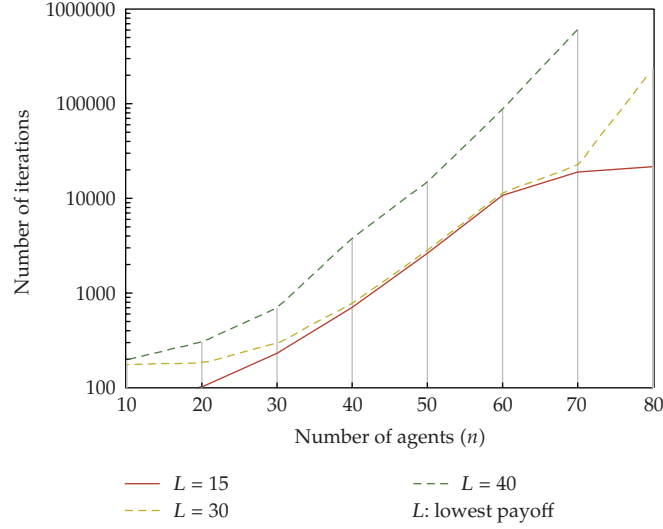
Figure 7: Number of iterations to equitable equilibrium as a function of L (lowest payoff) and n (number of agents); uncertainty parameter \varepsilon = 0.1 and memory length m = 10 .
