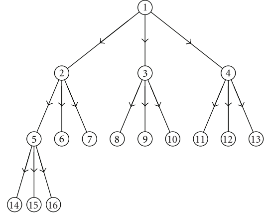
FIGURE 1: A directed rooted tree of 16 nodes.
