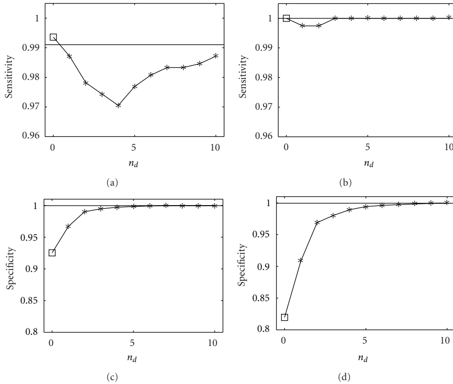
FIGURE 4: Sensitivity and specificity are plotted versus n_d , the number of variables selected for conditioning, for two values of the number of samples N , 500 (left) and 1000 (right). The order is m = 2 , similar results are obtained varying m . The results are averaged over 100 realizations of the linear dynamical system described in the text. The empty square, in correspondence to n_d = 0 , is the result from the bivariate analysis. The horizontal line is the outcome from multivariate analysis, where all variables are used for conditioning.
