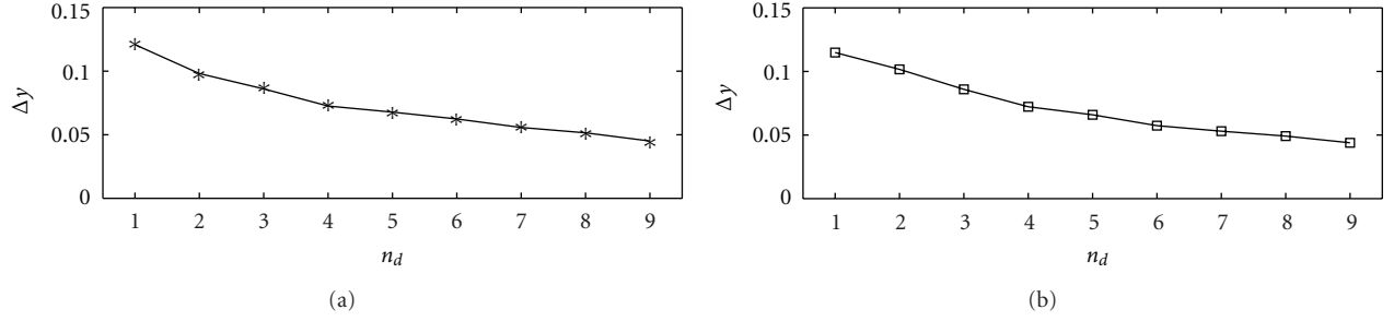
FIGURE 5: The mutual information gain, when the (n_d + 1) th variable is included, is plotted versus n_d for two values of the number of samples N , 500 (a) and 1000 (b). The order is m = 2 . The information gain is averaged over all the variables.
