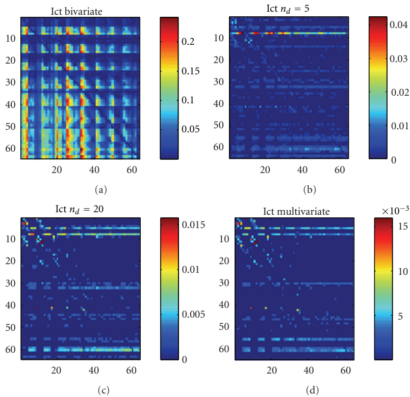
FIGURE 8: The sum of outgoing causality from each electrode in the EEG application, ictal period. (a) Bivariate analysis. (b) Our approach with n_d = 5 conditioning variables. (c) Our approach with n_d = 20 conditioning variables. (d) The multivariate analysis.
