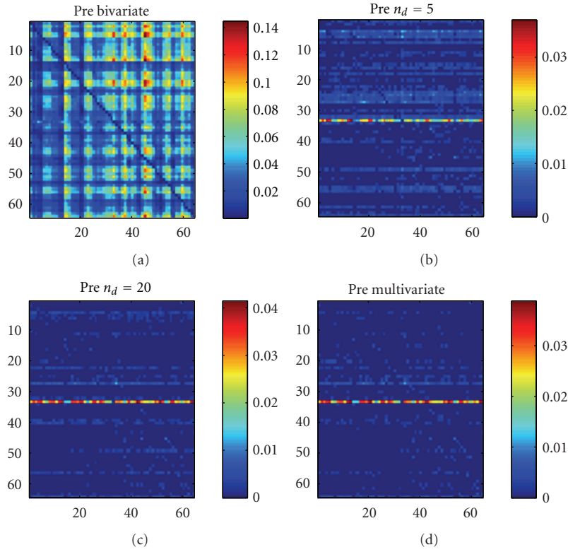
FIGURE 6: The causality analysis of the preictal period. The causality c(i \rightarrow j) corresponds to the row i and the column j . The order is chosen as m = 6 according to the AIC criterion. (a) Bivariate analysis. (b) Our approach with n_d = 5 conditioning variables. (c) Our approach with n_d = 20 conditioning variables. (d) The multivariate analysis.
