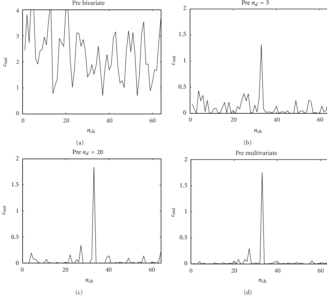
FIGURE 9: The sum of outgoing causality from each electrode in the EEG application, preictal period. (a) Bivariate analysis. (b) Our approach with n_d = 5 conditioning variables. (c) Our approach with n_d = 20 conditioning variables. (d) The multivariate analysis.
