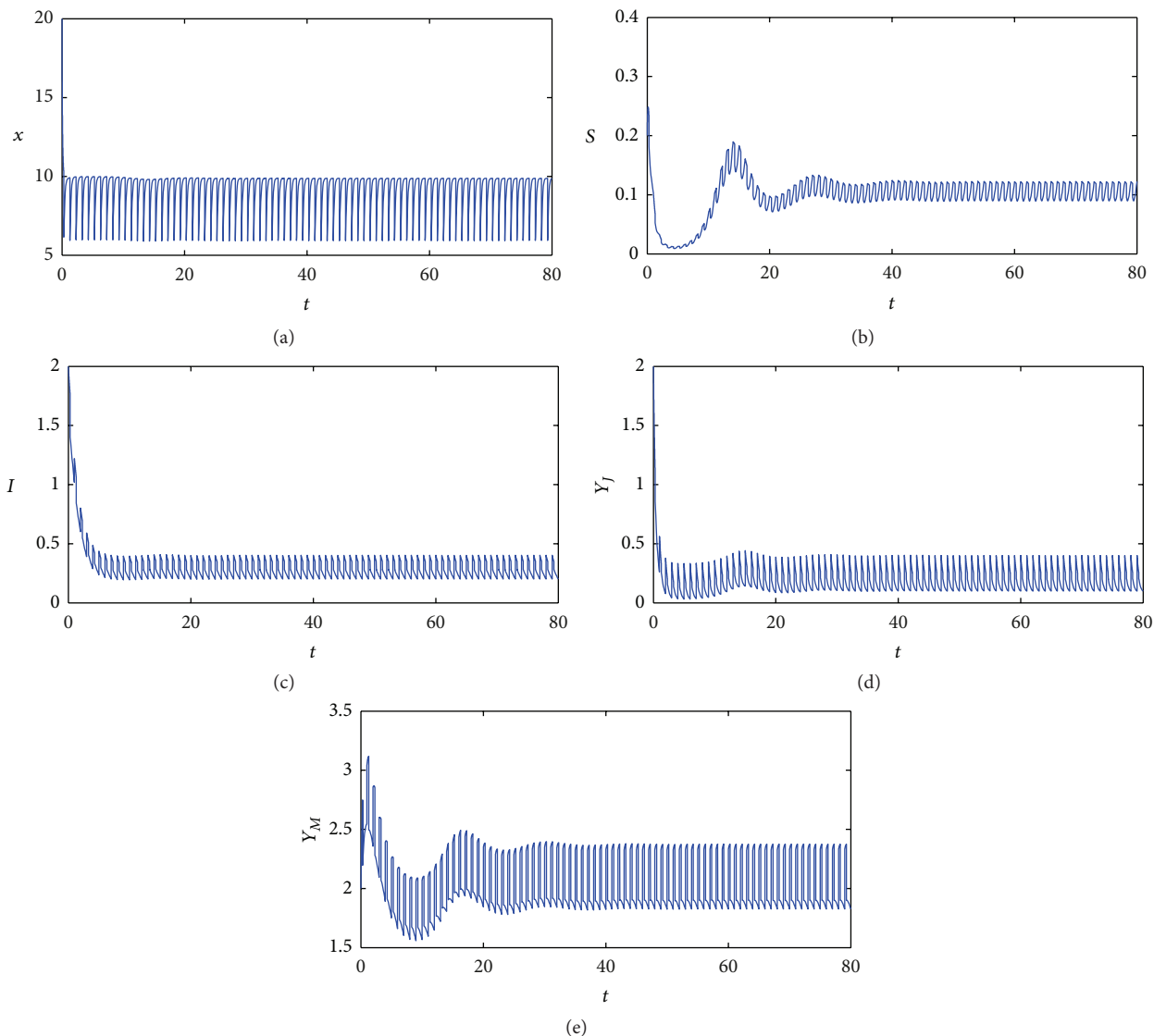
FIGURE 3: Time series of the system (68) with r = 8, K = 10, a = 0.8, \beta = 0.5, b = 0.3, h = 8, c = 0.2, \lambda = 0.6, m = 2, d_s = 0.2, d_I = 0.5, d_J = 0.4, d_M = 0.2, \delta = 0.4, P_S = P_I = P_J = P_M = 0.2, \delta_I = 0.2, \delta_J = 0.3, \delta_M = 0.5, \tau = 0.3, T = 1, x(0) = 20, S(0) = 0.2, I(0) = 2, y_j(0) = 2, y_M(0) = 2 .
