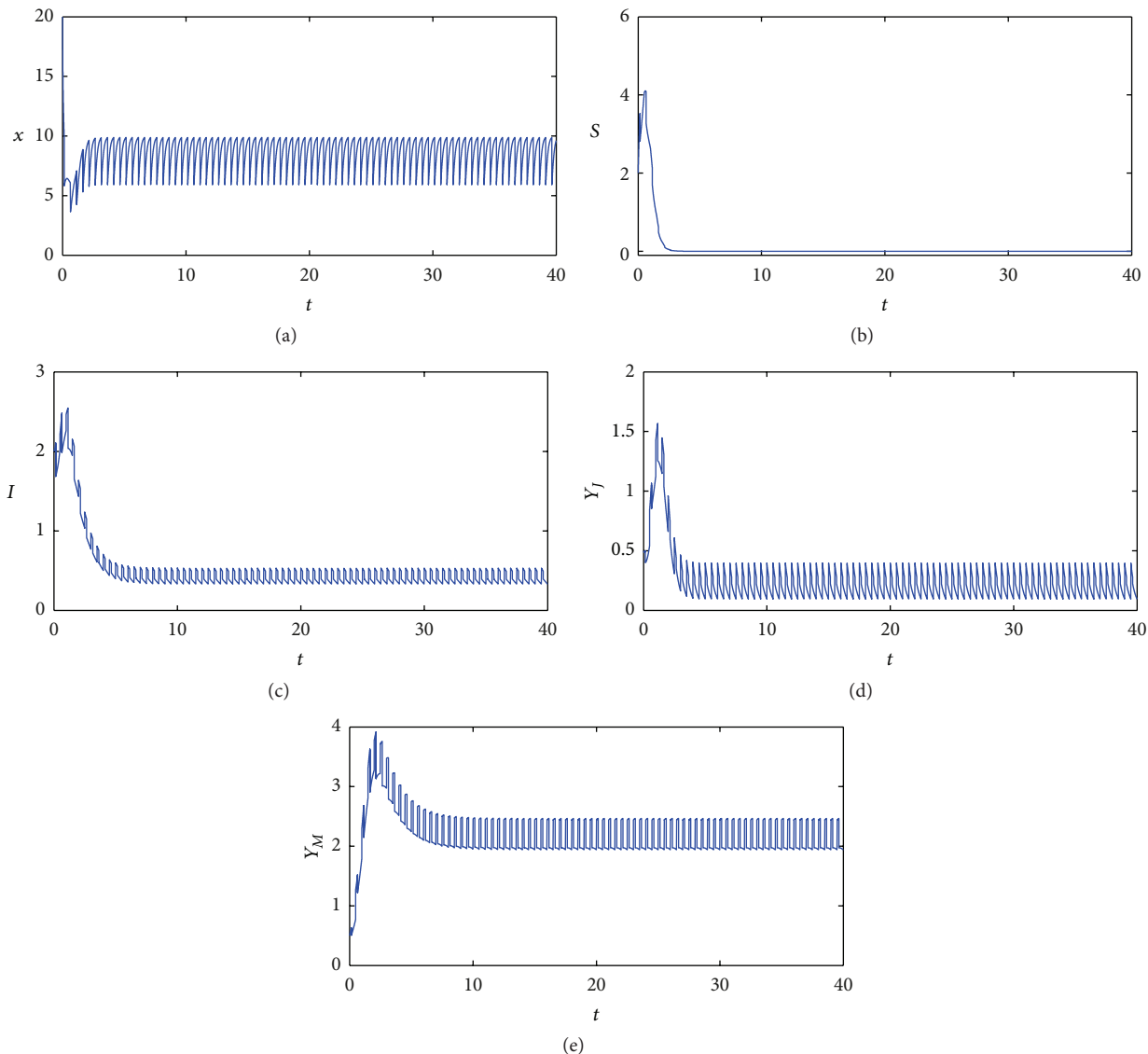
FIGURE 1: Time series of the system (68) with r = 8, K = 10, a = 0.8, \beta = 0.5, b = 0.3, h = 8, c = 0.2, \lambda = 0.6, m = 2, d_s = 0.2, d_I = 0.5, d_J = 0.4, d_M = 0.2, \delta = 0.4, P_S = P_I = P_J = P_M = 0.2, \delta_I = 0.2, \delta_J = 0.3, \delta_M = 0.5, \tau = 0.3, T = 0.5, x(0) = 20, S(0) = 2, I(0) = 2, y_j(0) = 0.5, y_M(0) = 0.5 .
