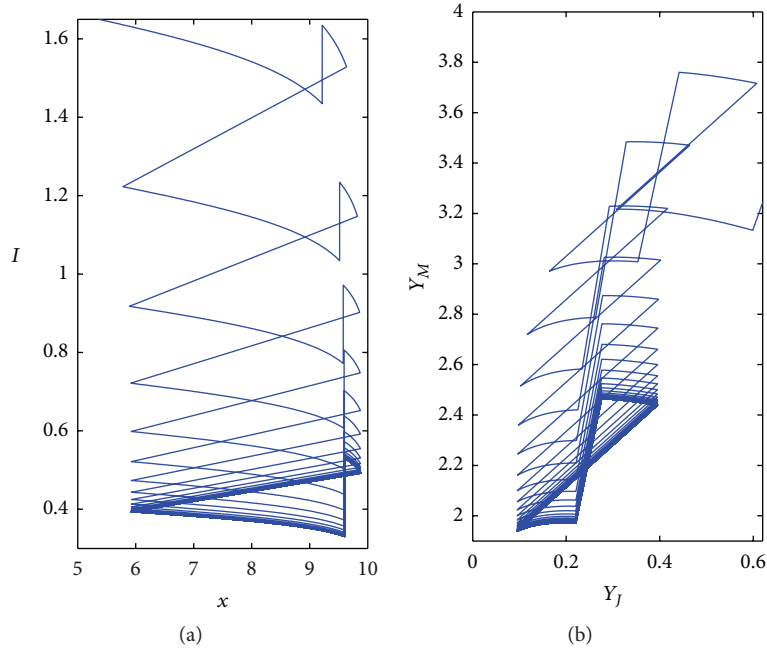
FIGURE 2: Phase portrait of the system (68) with r = 8, K = 10, a = 0.8, \beta = 0.5, b = 0.3, h = 8, c = 0.2, \lambda = 0.6, m = 2, d_S = 0.2, d_I = 0.5, d_J = 0.4, d_M = 0.2, \delta = 0.4, P_S = P_I = P_J = P_M = 0.2, \delta_I = 0.2, \delta_J = 0.3, \delta_M = 0.5, \tau = 0.3, T = 0.5, x(0) = 20, S(0) = 2, I(0) = 2, y_j(0) = 0.5, y_M(0) = 0.5 .
