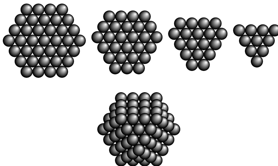
Figure 8. A half-cuboctahedron block, exploded into layers and assembled
